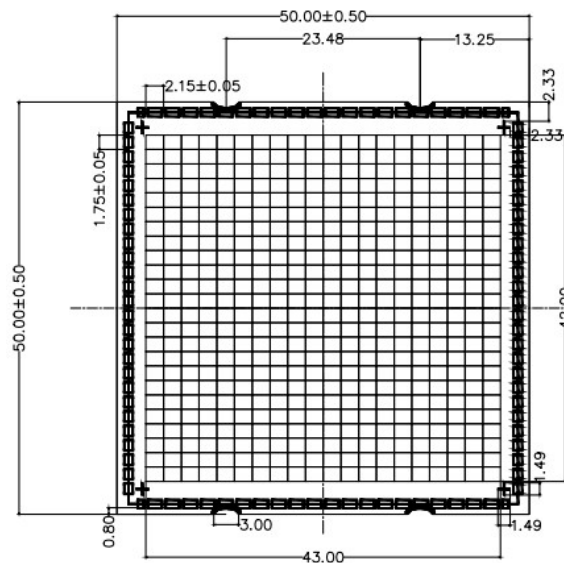
ARRAY LAYOUT [20X24=480PCS/ARRAY SHEET]
